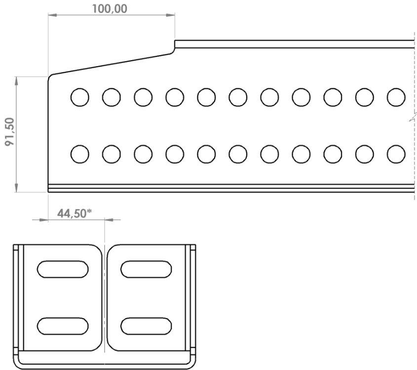
Universal front cut
