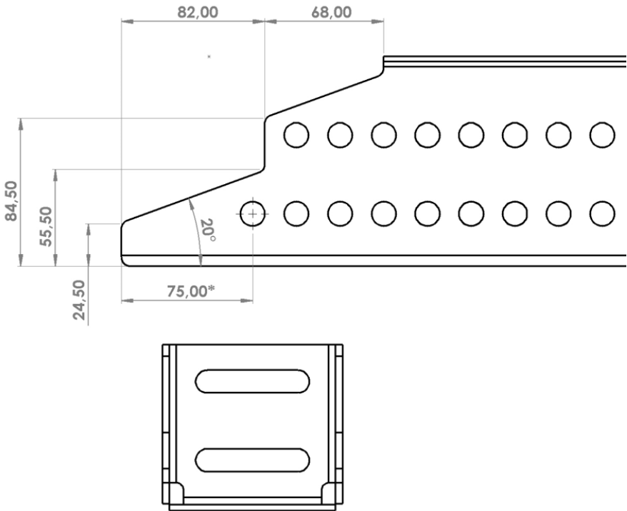
Front cut IVECO Daily
