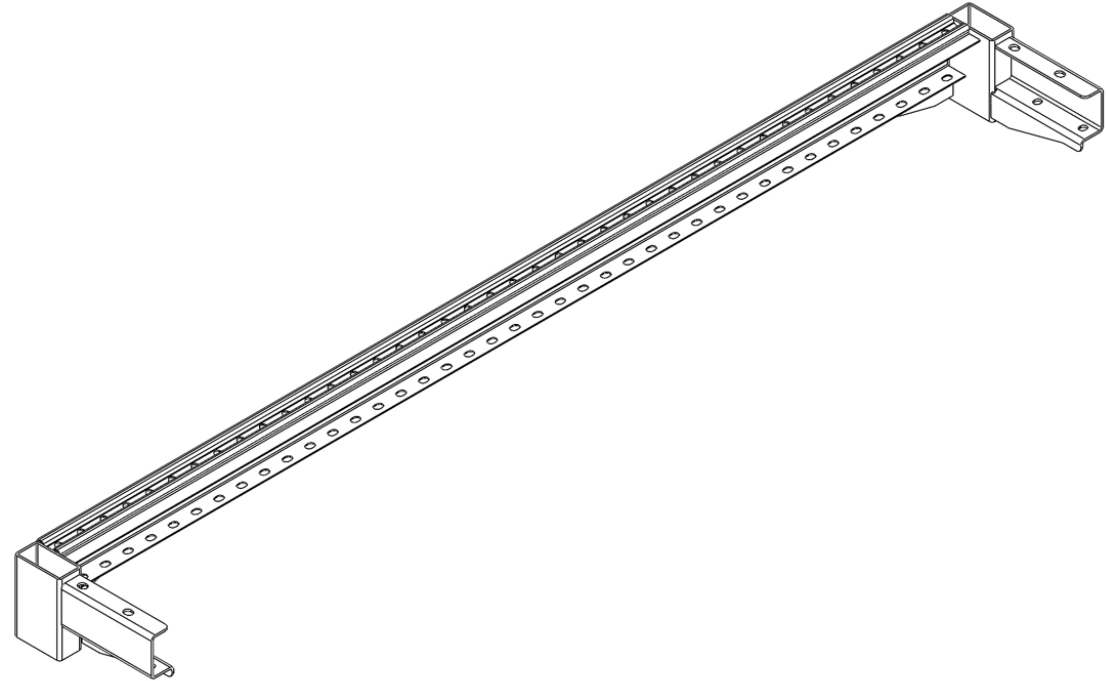
Front/rear traverse S355MC
