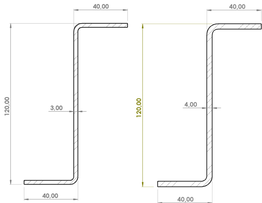
Longitudinals Z 120/30/3 mm S355MC
