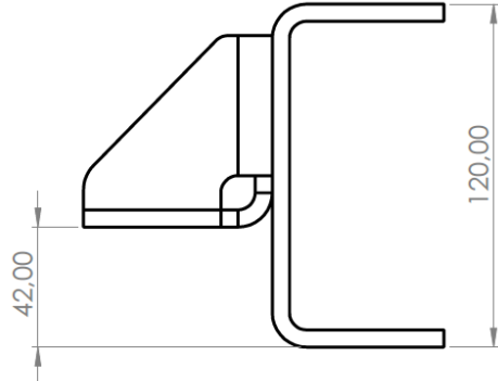
Bracket 135x67-6 mm Upper position
