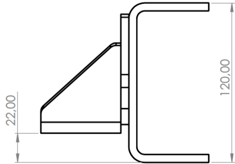
Bracket wide 218x90-6 mm
