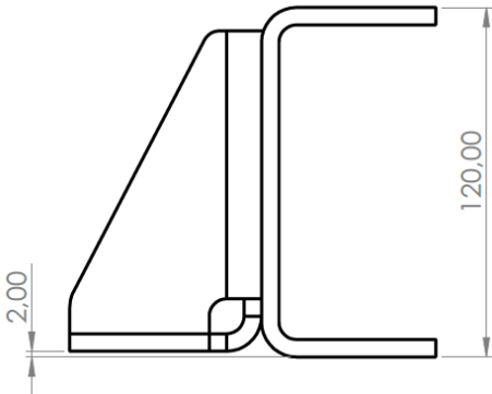
Bracket 135x110-6 mm
