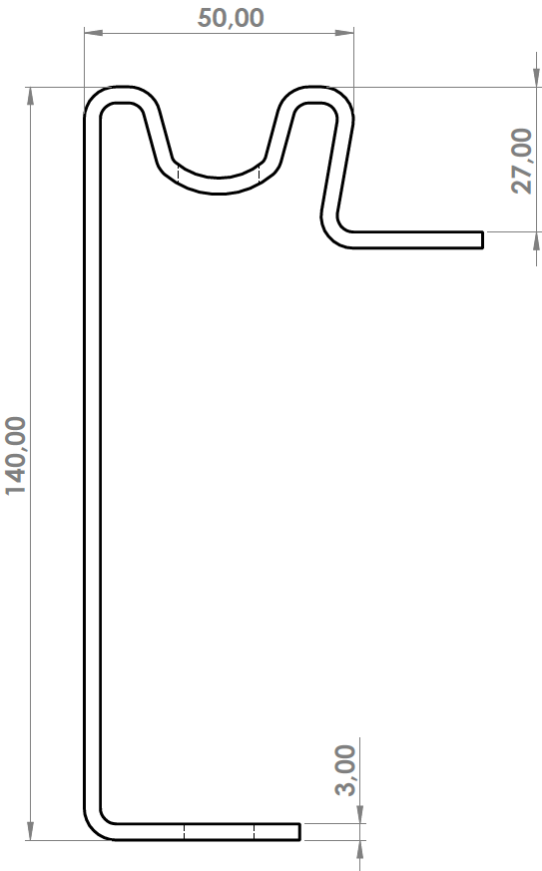
Side rave profile UL 140/27/3 mm S355MC
