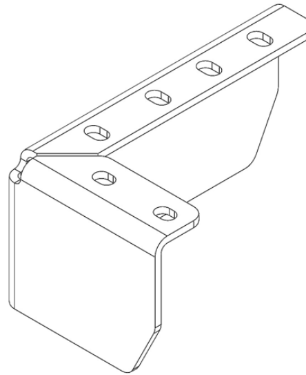
Corner extender 265x150x125-6 mm L/P S355MC
