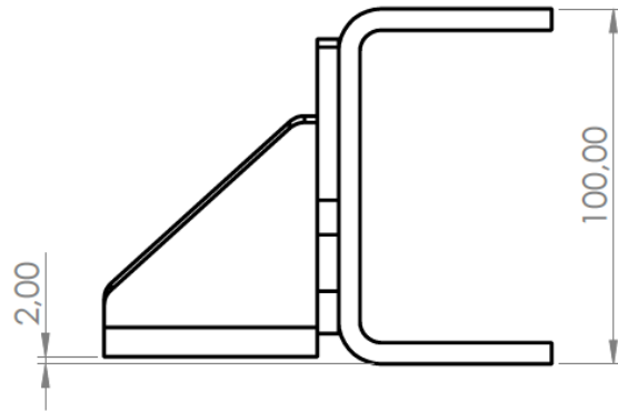
Bracket wide 218x90-6 mm
