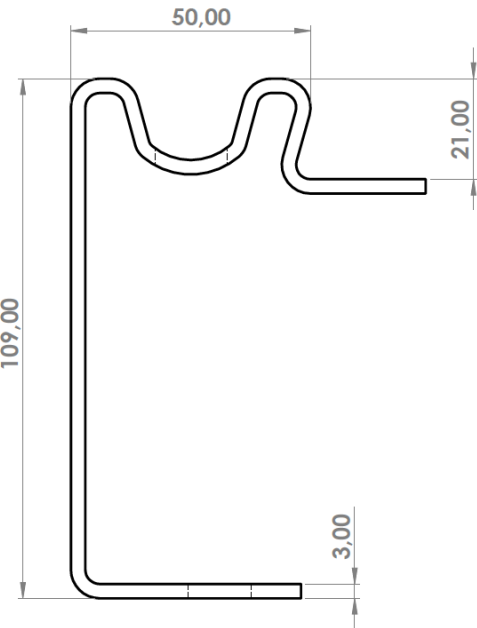
Side rave profile UL 109/21/3 mm S355MC
