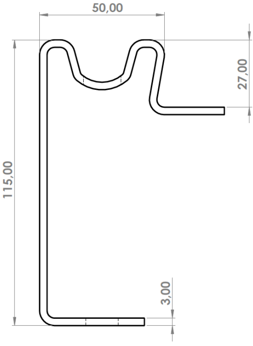
Side rave profile UL 115/27/3 mm S355MC
