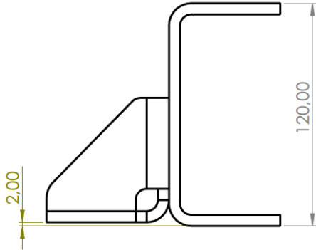
Bracket 135x67-6 mm Lower position
