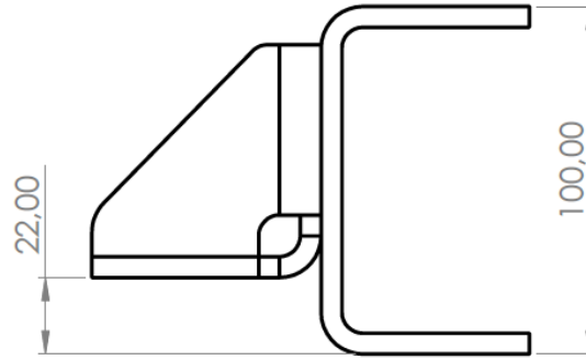
Bracket 135x67-6 mm
