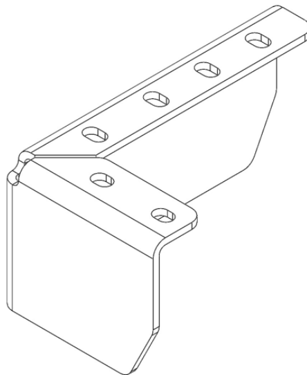
Dolní roh 265x150x125-6 mm L/P S355MC
